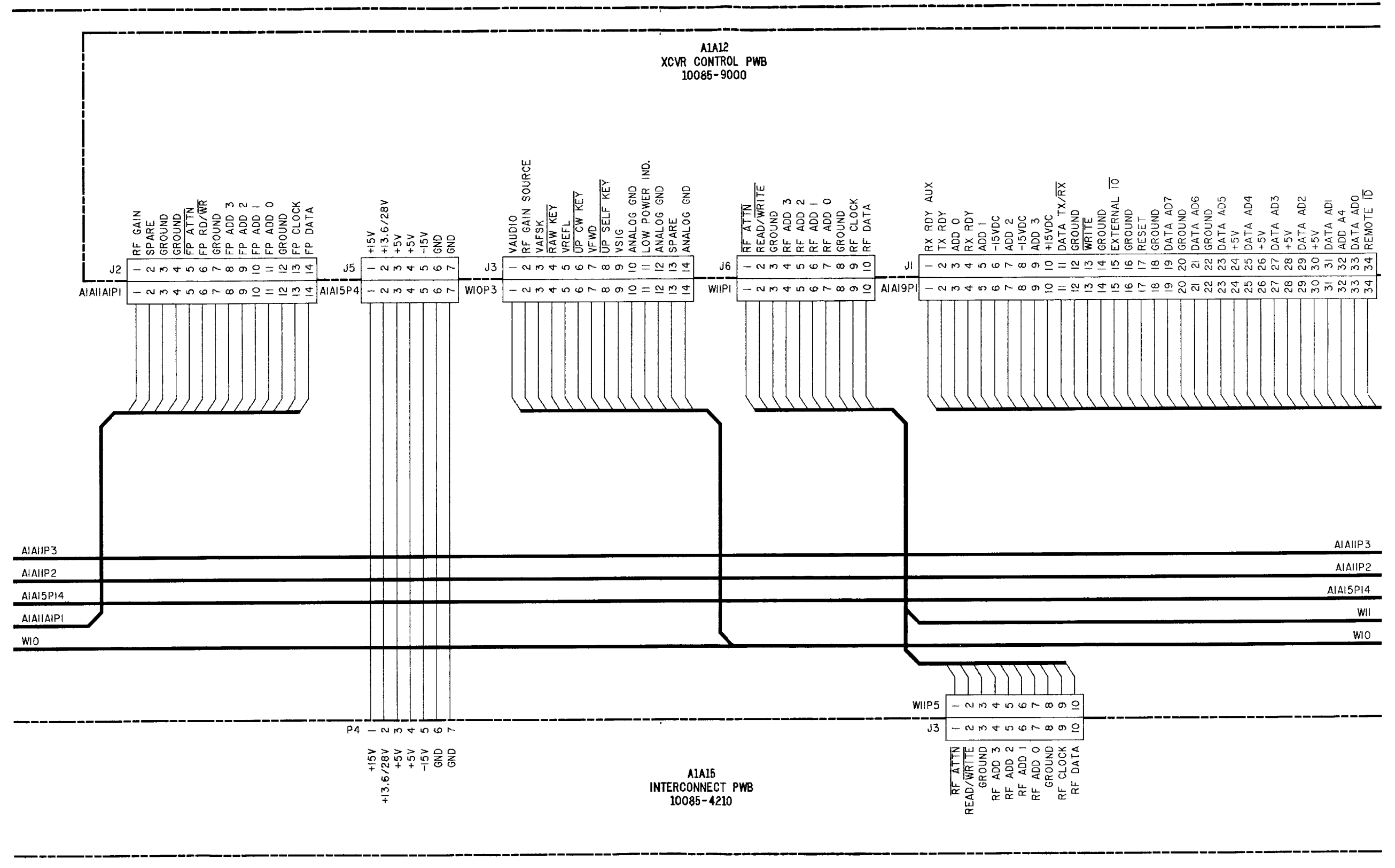
FO-2. TRANSCIVER ASSY, A1, INTERCONNECTION DIAGRAM (Sheet 2 of 13)
